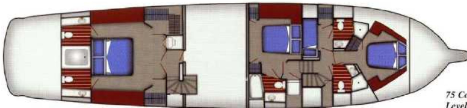
75 Cockpit Upper Level Arrangement
